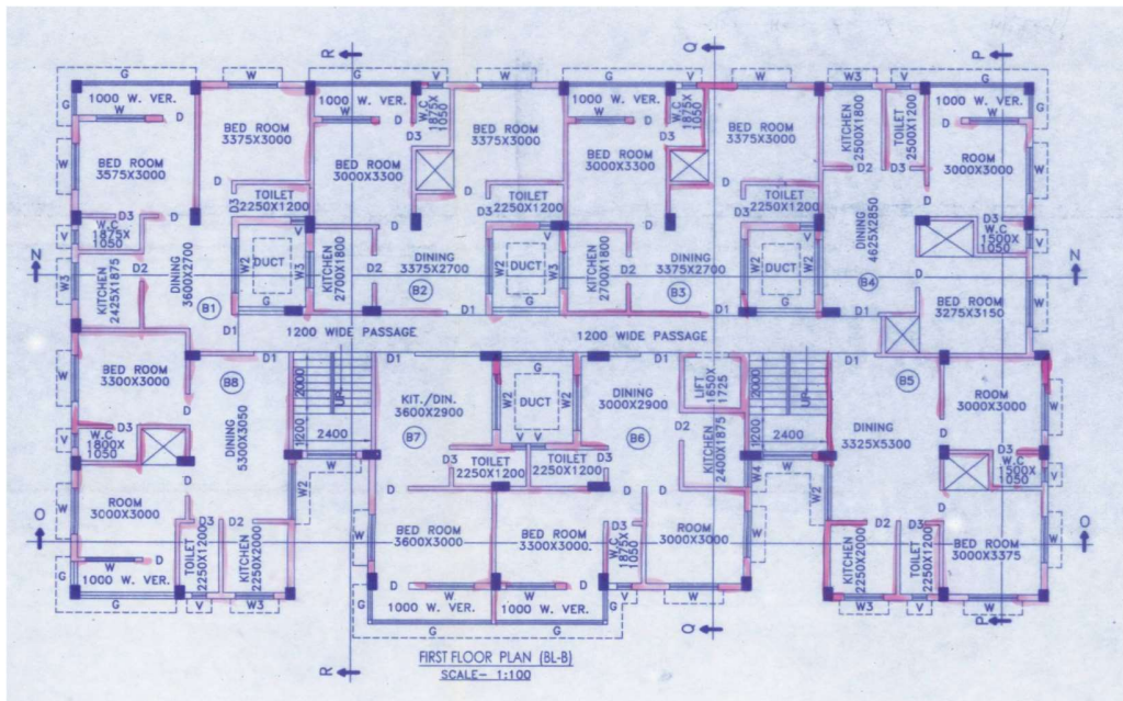
Block-A 1 st Floor Plan
