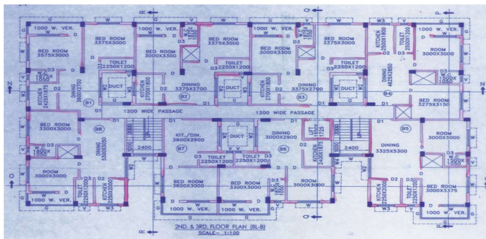
Block-A 2 nd & 3 rd Floor Plan
